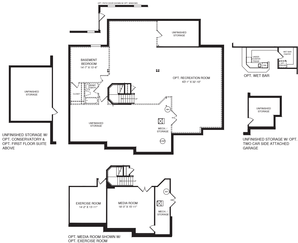
LOWER LEVEL
