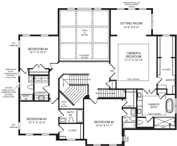
UPPER LEVEL
