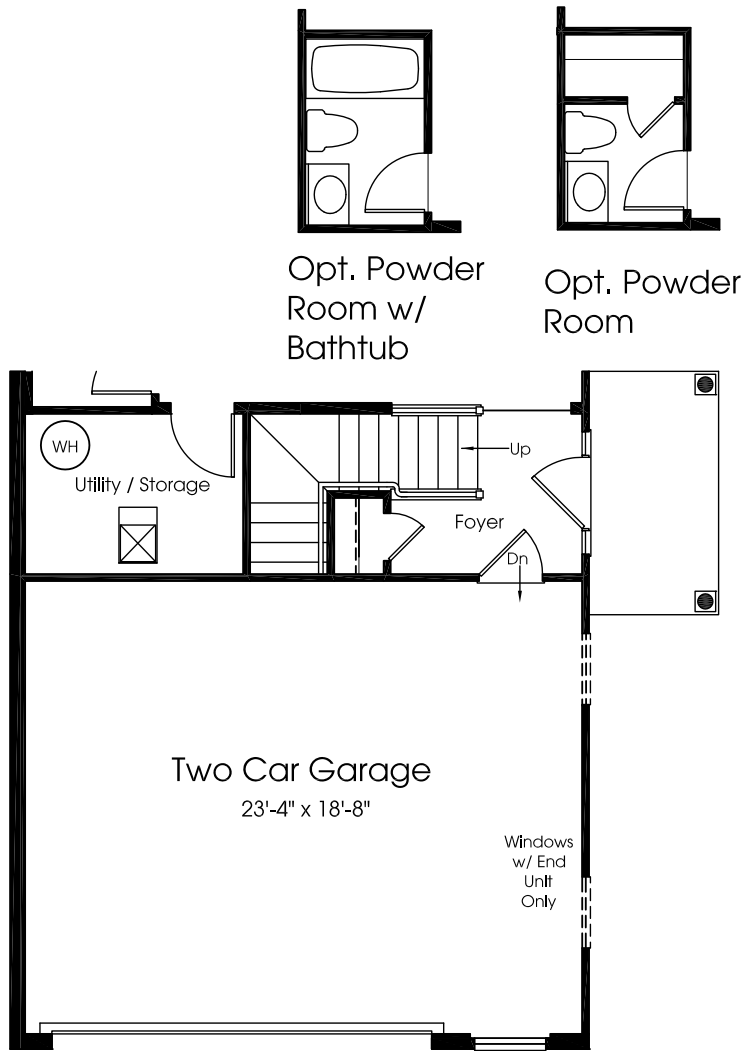
Side Entry
