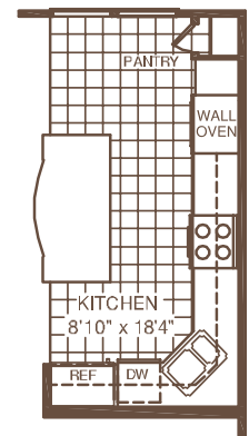
OPT. GOURMET KITCHEN W/ OPT. 4'-0" EXTENSION
