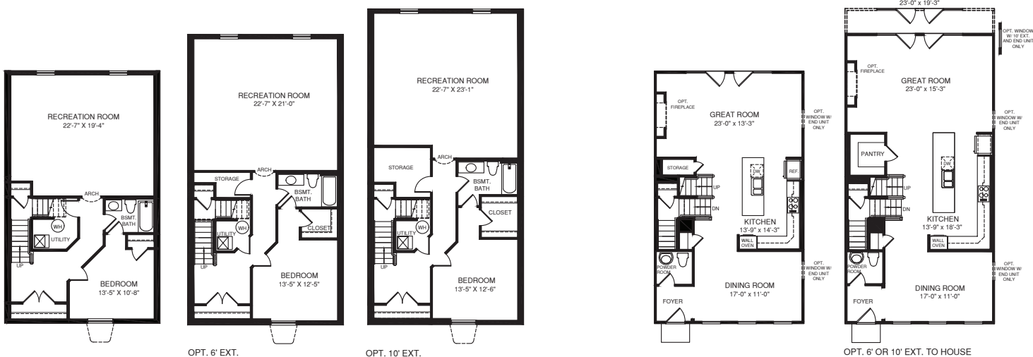
MAIN LEVEL
