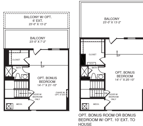
ATTIC LEVEL
