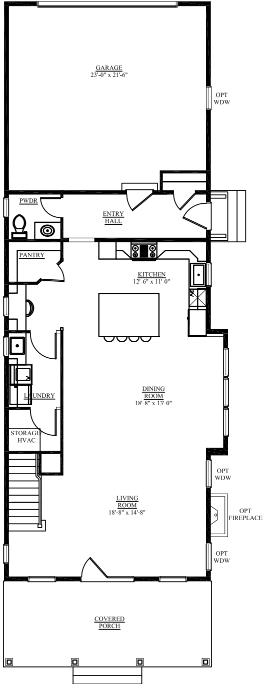
MAIN LEVEL TWO CAR REAR GARAGE - GCD
