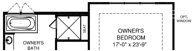
OPT. 4'-0" EXTENSION TO OWNER'S BEDROOM
