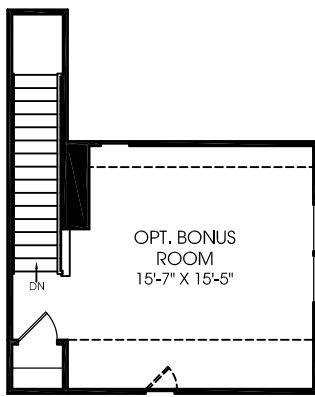
ACCESS DOOR W/ OPT. ATTIC STORAGE OPT. BONUS ROOM
