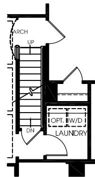
FIRST FLOOR STAIRS W/ OPT. BONUS ROOM / BEDROOM
