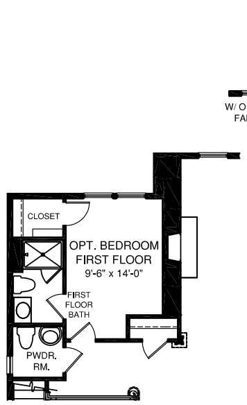
OPT. BEDROOM FIRST FLOOR SHOWN W/ OPT. ENTERTAINMENT CENTER
