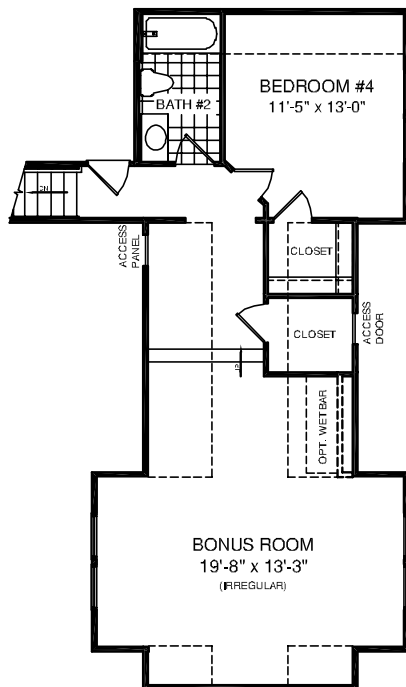
OPT. BONUS ROOM & OPT. BEDROOM
