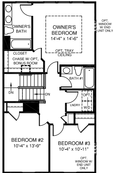
OPT. OWNER'S BATH
