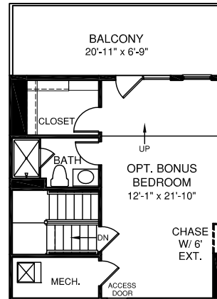
OPT. BONUS LEVEL
