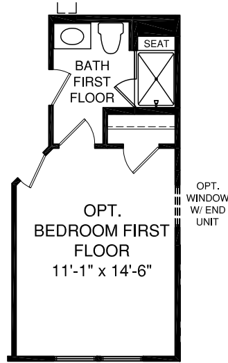
OPT. BEDROOM FIRST FLOOR & BATH
