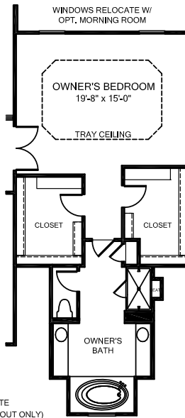
ALTERNATE OWNER'S BEDROOM LAYOUT W/ OPEN FAMILY ROOM (AVAILABLE W/ ALL 2ND FLOOR PLANS)
