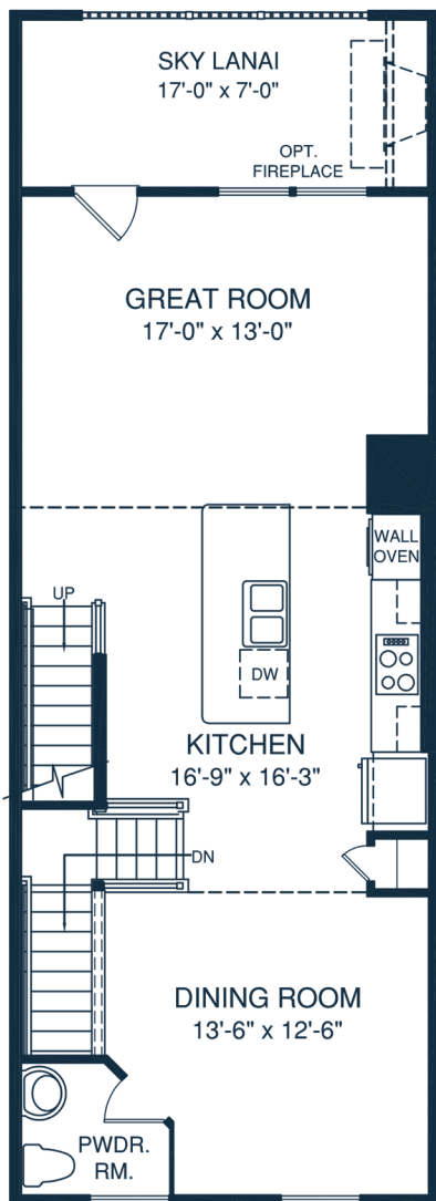
MAIN LEVEL
