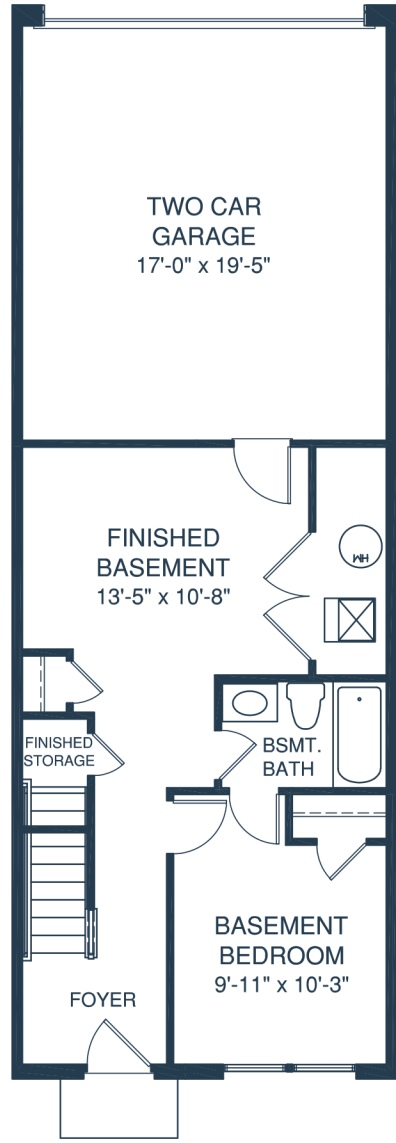
REAR-LOAD GARAGE
