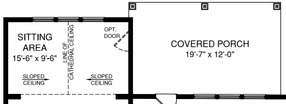
OPT. SITTING AREA SHOWN W/ OPT. COVERED PORCH
