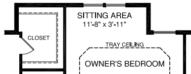
OWNER'S BEDROOM W/ OPT. 4' EXT. TO HOUSE
