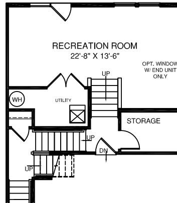
OPT. 4' STEP DOWN ALSO AVAILABLE W/ 6' OR 10' EXT. SEE BLUEPRINTS FOR DETAILS.
