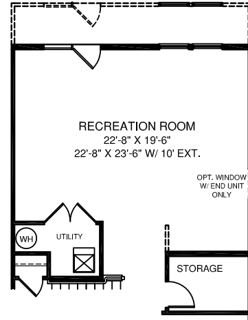
OPT. 6' OR 10' EXT.
