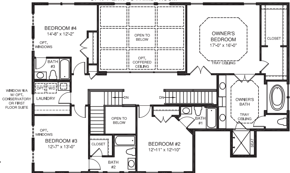
OPT. 4' EXT. TO FAMILY ROOM
