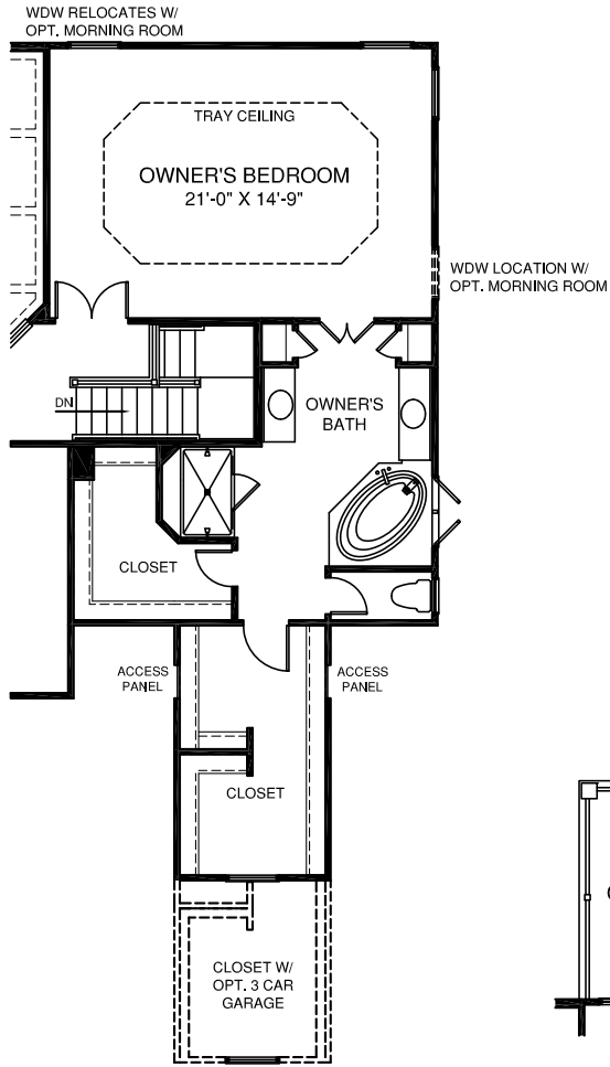
OWNER'S BATHROOM ALTERNATE LAYOUT
