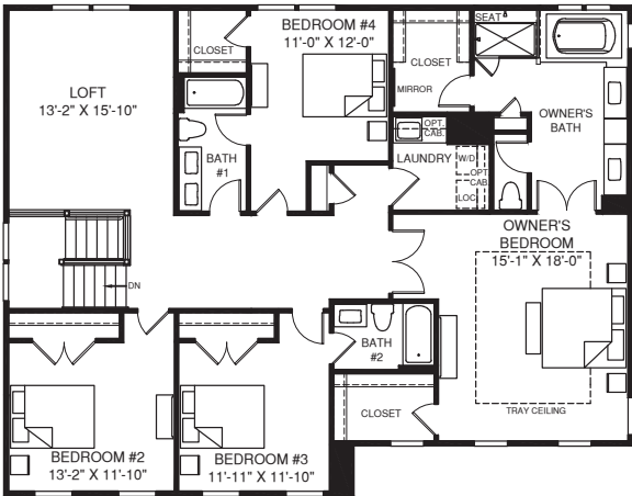
FOUR BEDROOM W/ OPT. LOFT
