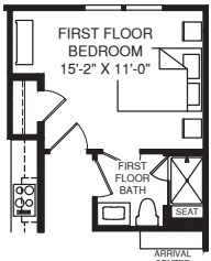
OPT. FIRST FLOOR BEDROOM
