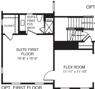
OPT. FIRST FLOOR SUITE
