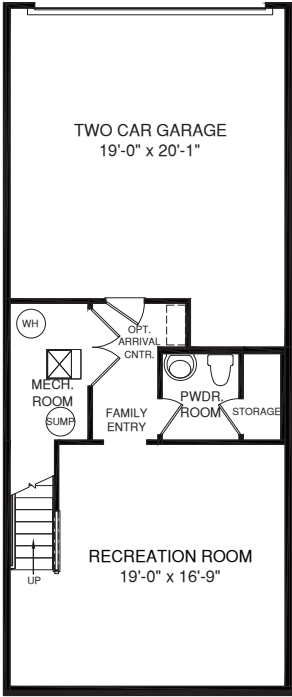
LOWER LEVEL
