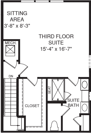
OPT. THIRD FLOOR SUITE
