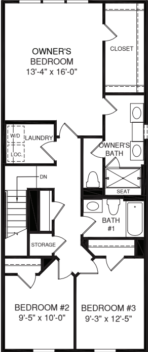
SECOND FLOOR
