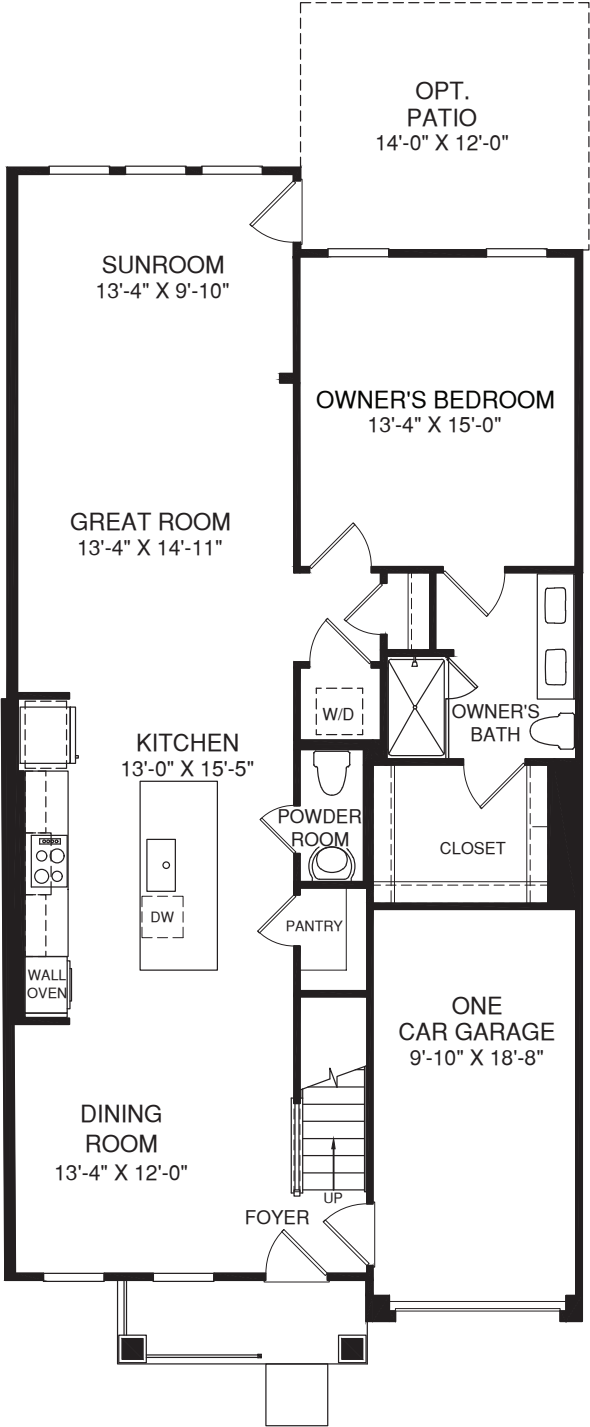
MAIN LEVEL
