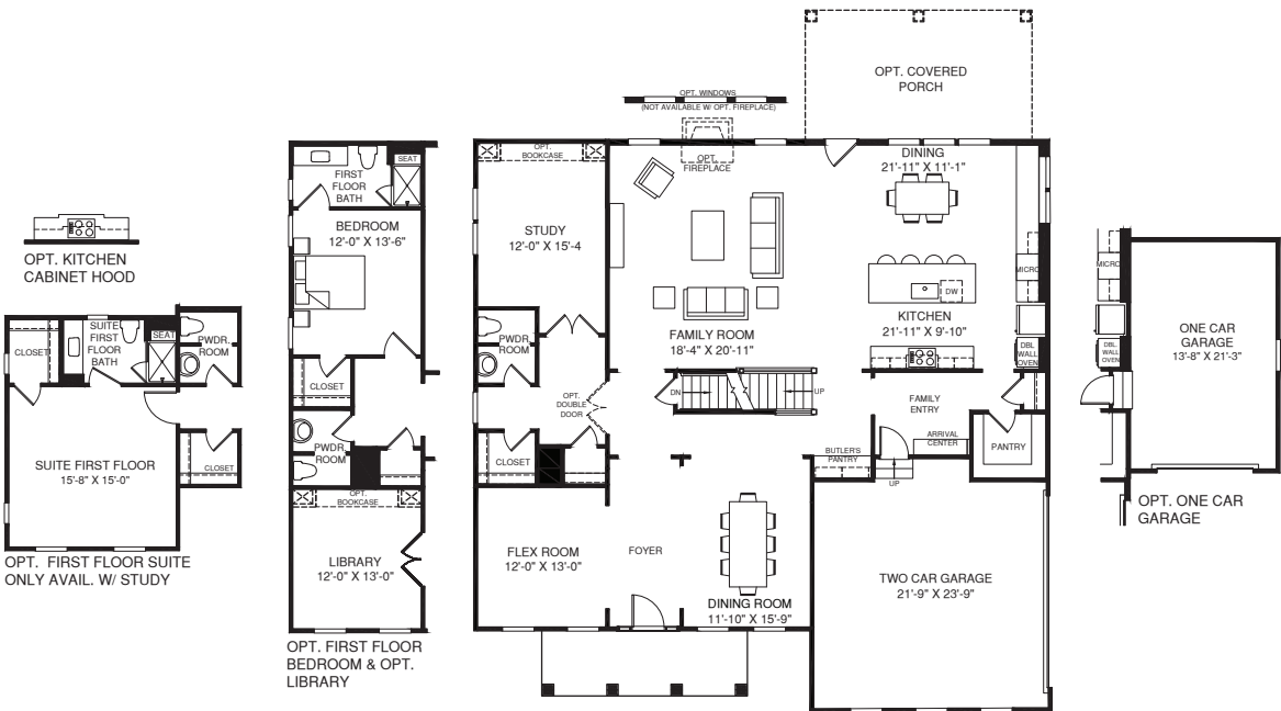
MAIN LEVEL
