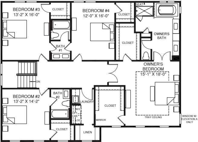
OPT. OWNER'S BATHROOM FREESTANDING TUB & ROMAN SHOWER
