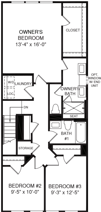
THIRD FLOOR
