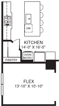
OPT. KITCHEN CABINET HOOD SHOWN W/ OPT. FLEX ROOM
